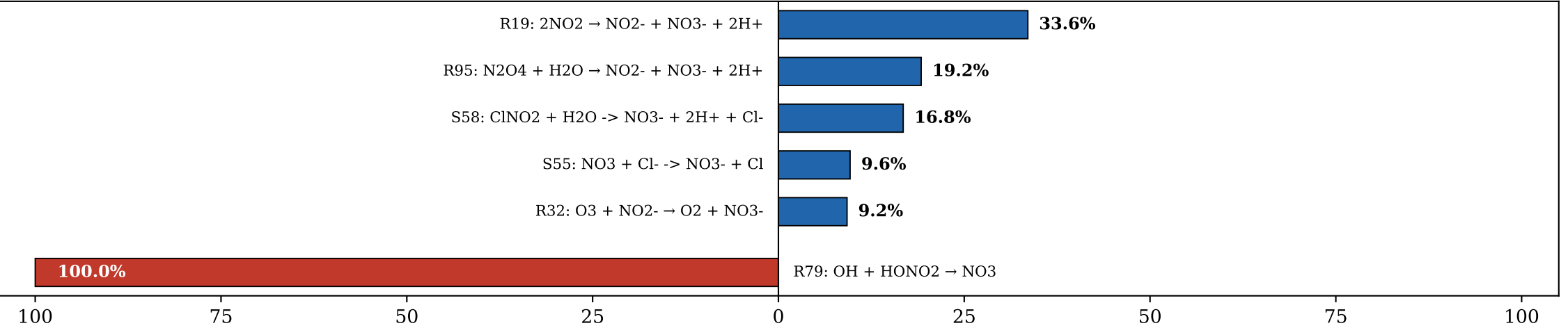
(b) O 3 (Σsrc = 1.30e-07 M/s)
