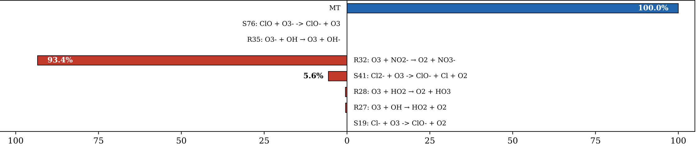
(c) NO 2 - (Σsrc = 3.34e-07 M/s)
